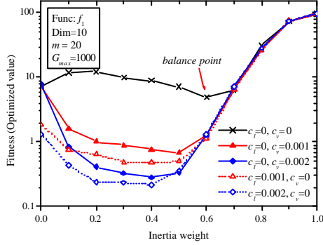
FIG. 1 10-D Rastrigrin function with different c_v and c_l
